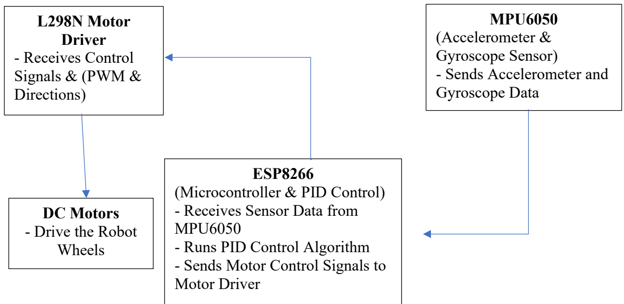
Fig. 1. Self-Balancing Block Diagram
